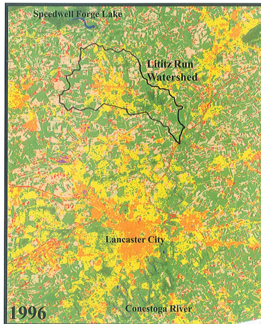
Comparison of the 1987 image (left) with the 1996 image (right) shows a significant increase in suburban development both within the watershed and throughout Lancaster County. Suburban sprawl is a serious problem facing the watershed, Lancaster County and areas throughout the nation. (Landsat TM satellite images: classification by LandStudies, Inc., Warwick Township and Penn State Department of Meteorology)
