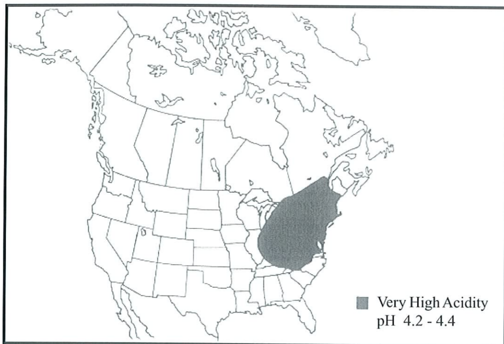
Map showing area in northeastern United States and southeastern Canada with precipitation that ranges in pH from 4.2 to 4.4 (from Miller 1995)
