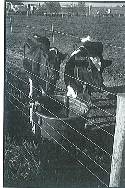
Solar pumps (above) and spring development watering systems can eliminate the need for livestock to access the stream. Concrete stream crossings (right) increase the health and safety of livestock while reducing streambank erosion. (Photo: Frank Lucas, Pequea-Mill Creek Project)
