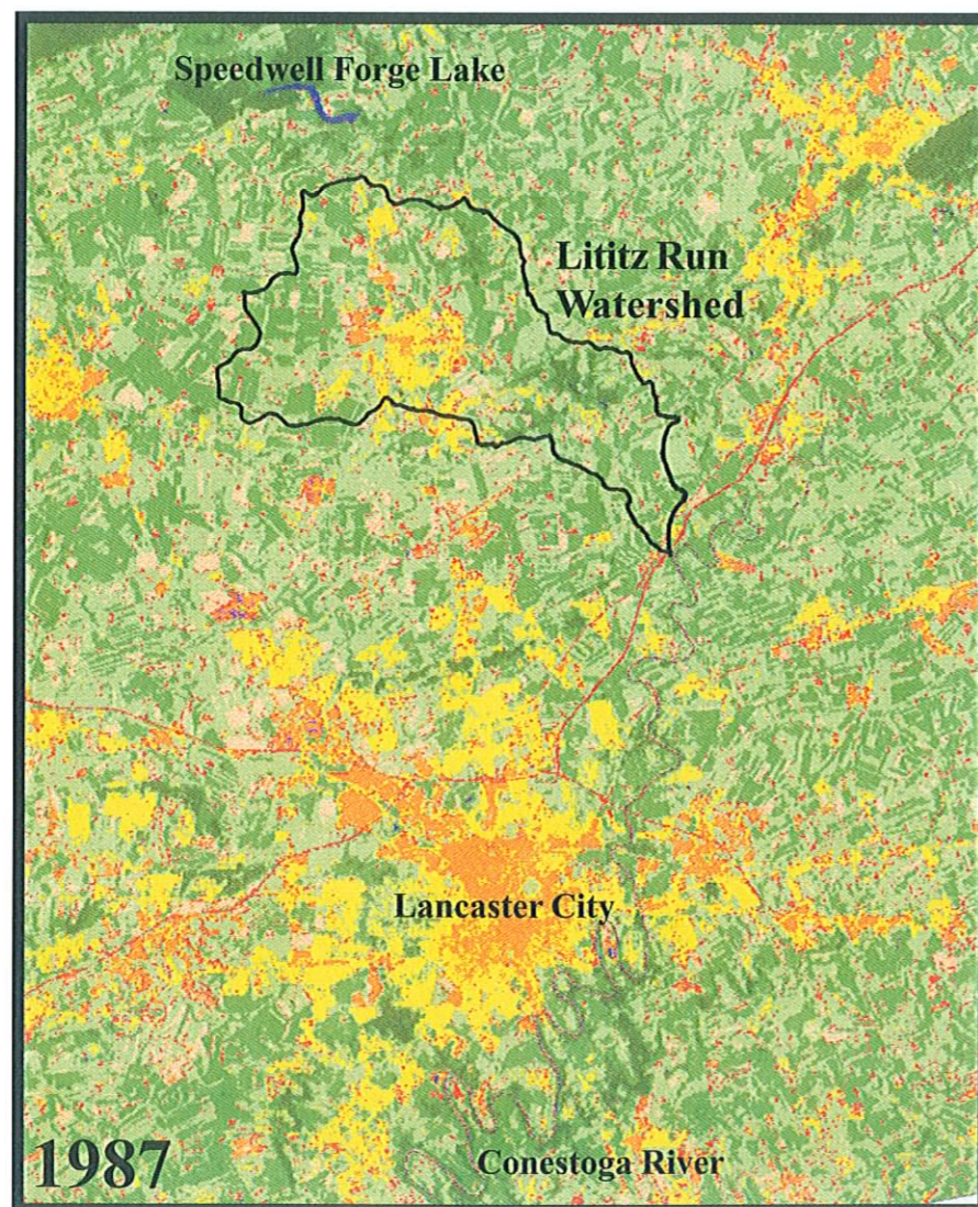
Satellite images showing different land surface classifications. These classifications are: Orange- downtown / urban areas, Yellow- suburban areas, Red- developed areas / highways, Light Green- agricultural crops / pasture, Tan- bare soil / cultivated agricultural fields, Purple- rock / quarries, Dark Green- woodlands and Blue- water. The Lititz Run Watershed is outlined and located in the upper-center of the image.
