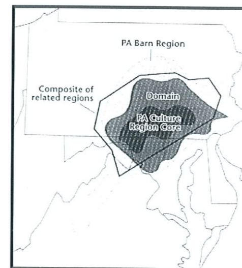
Map of Middle Atlantic States showing the Pennsylvania Culture Region Core in dark. (Zelinsky 1995)
